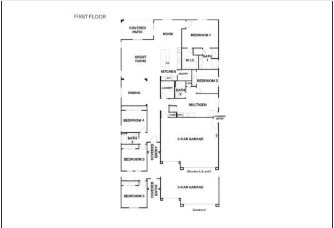
Floor Plan 1
