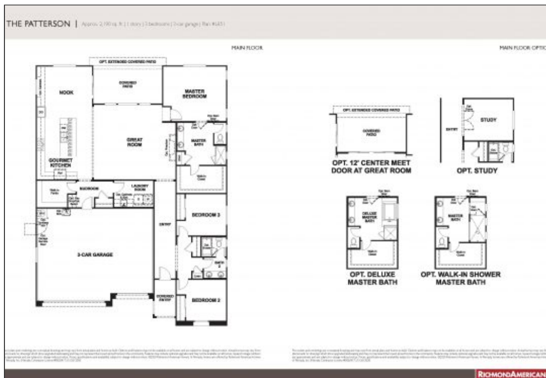
Floor Plan 1
