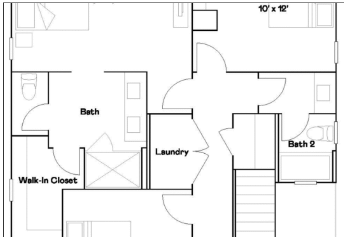
Floor Plan 2
